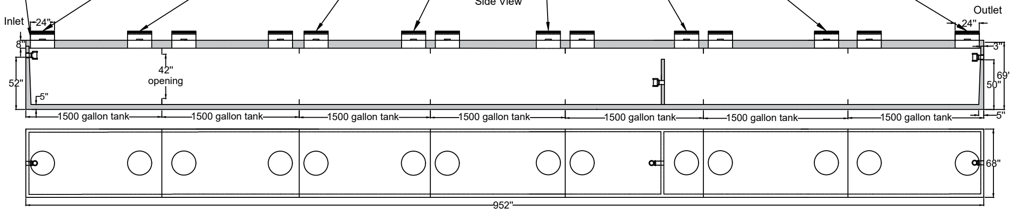
Top View (covers removed)
