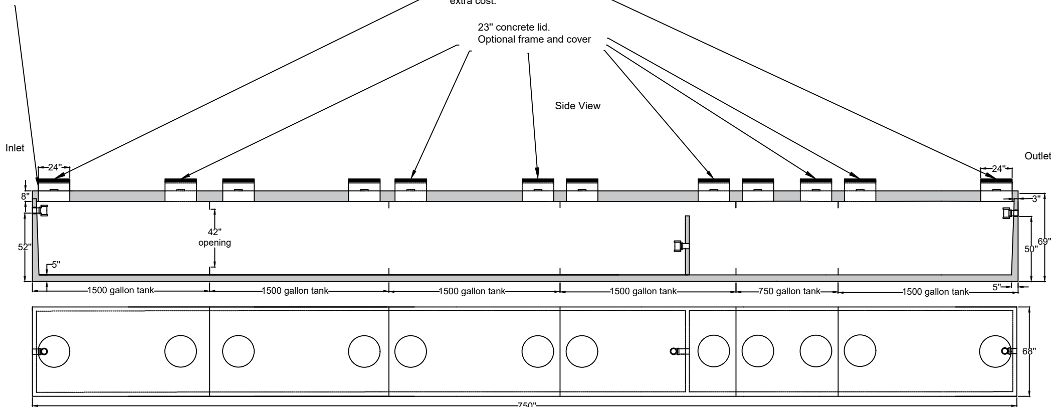
Top View (covers removed)
