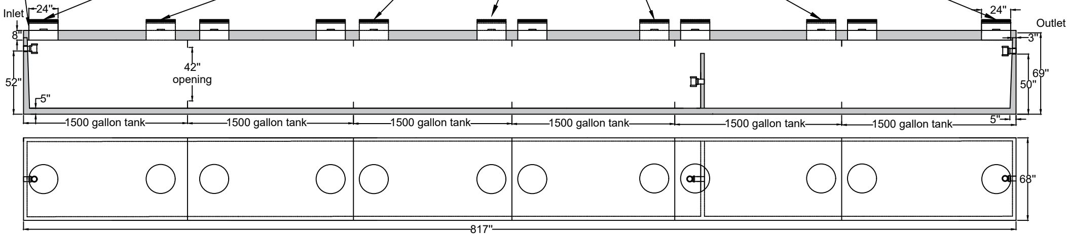
Top View (covers removed)
